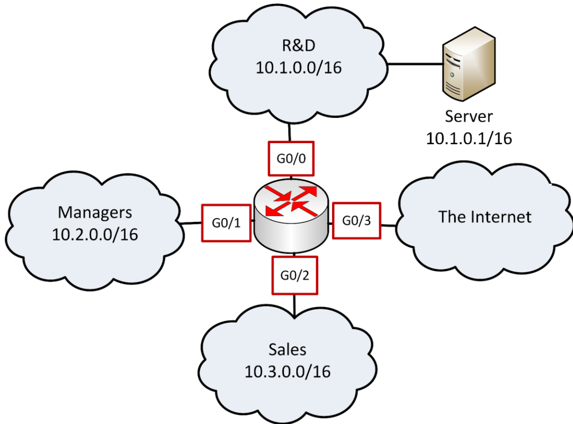
Diagram 9: Extended IP access-control lists
