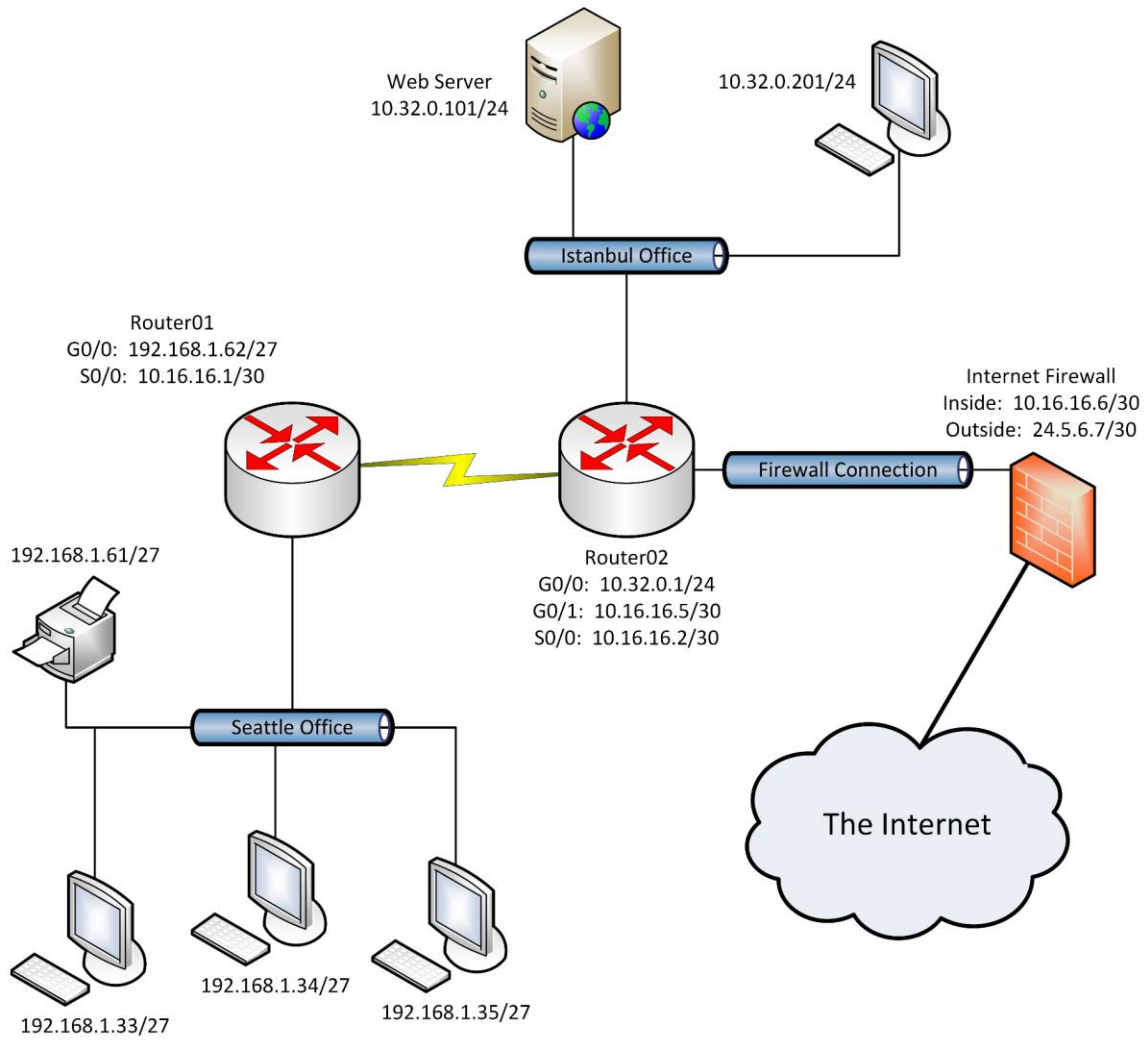
Diagram 8: Stand IP access-control lists, part 2
