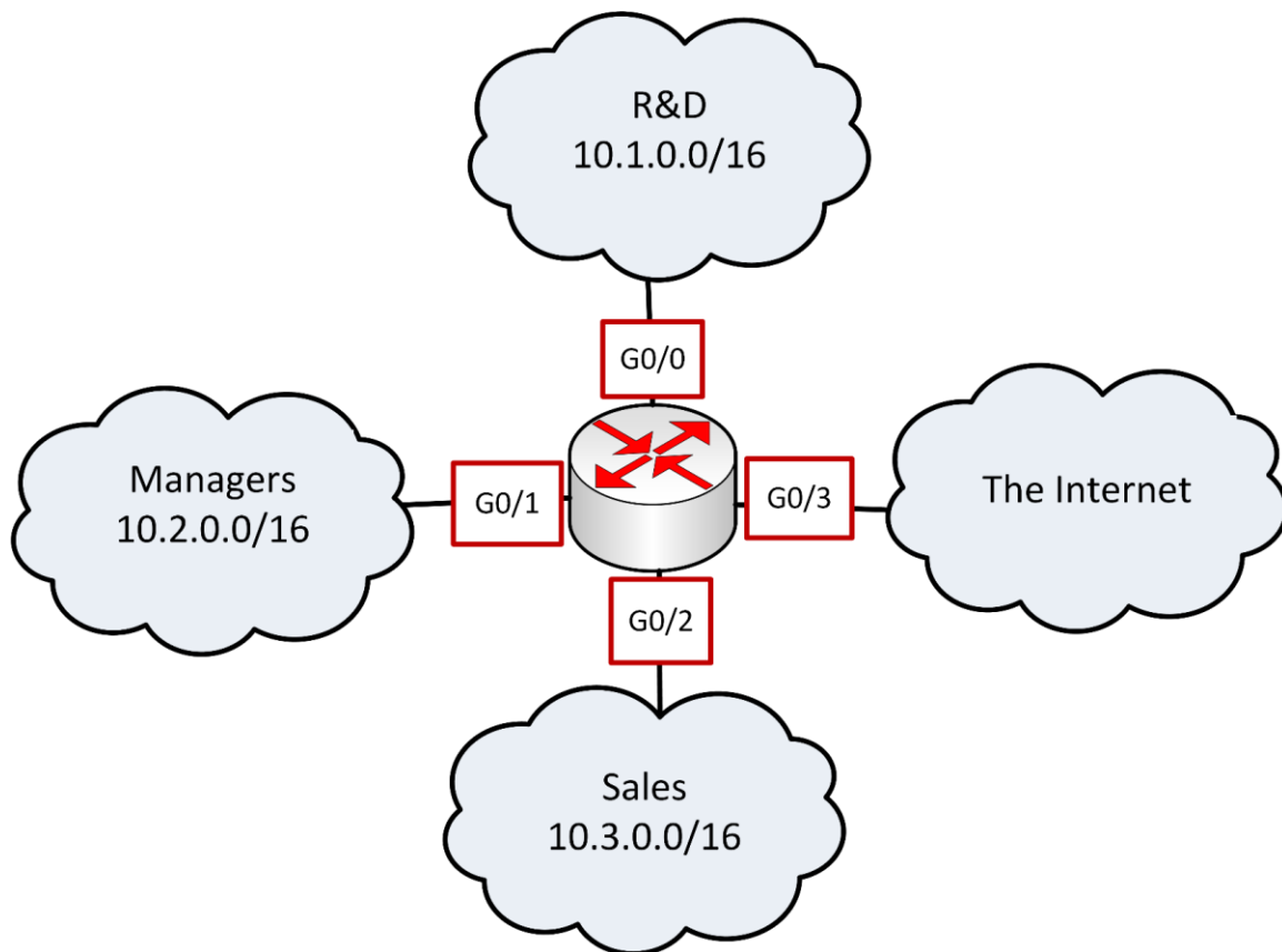
Diagram 7: Stand IP access-control lists
